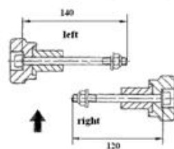
Installation position ( torque 50 Nm )
